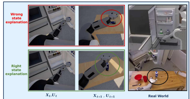
Fig. 13: NaivPhys4RP explains future desired state of world.
