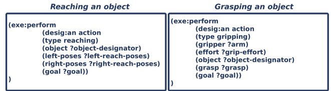
Fig. 10: Underspecified primitive action plans.
