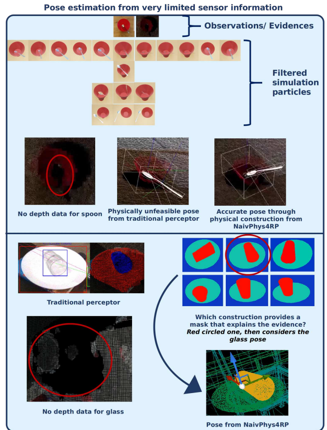
Fig. 12: NaivPhys4RP estimates poses from poor depth.
