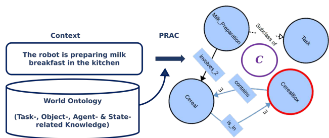
Fig. 8: Context formalization.
