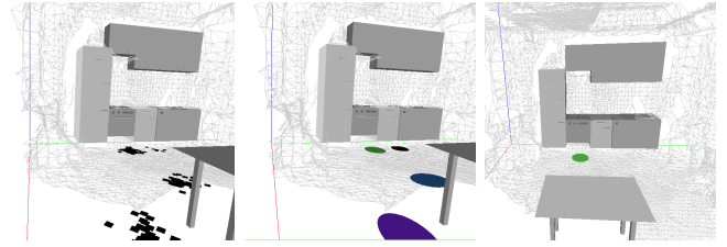
Fig. 4. Observed positions of manipulation actions (left), the positions clustered into places (center), and the result that has been learned as the “place for picking up pieces of tableware” (right). The pictures are visualized results of queries to the knowledge processing system.
